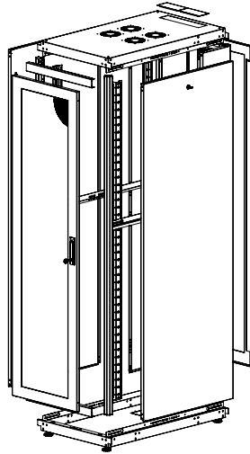
EXPLODED VIEW
