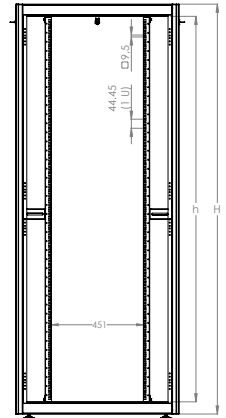
DIMENSIONS IN WIDTH AND HEIGHT
