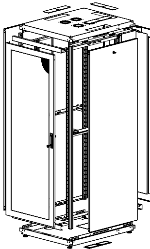
EXPLODED VIEW
