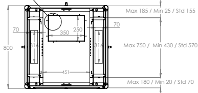
MAX/STD/MIN EQUIPMENT MOUNTING DISTANCE
