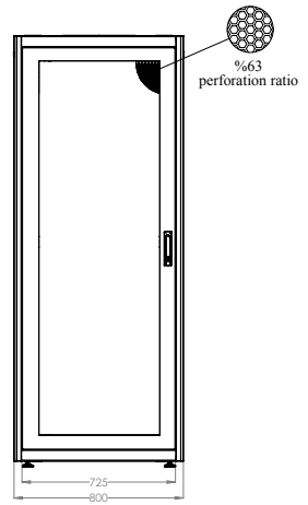
REAR VIEW
