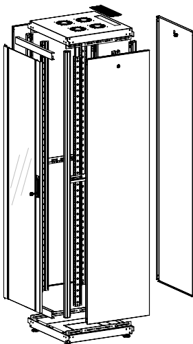
EXPLODED VIEW
