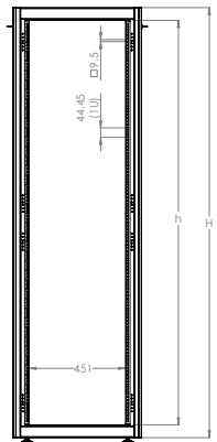
DIMENSIONS IN WIDTH AND HEIGHT
