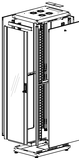
EXPLODED VIEW
