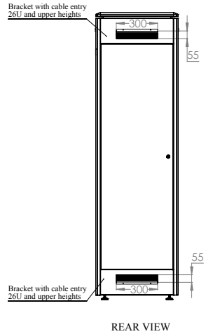
REAR VIEW
